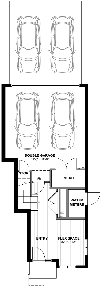
MAIN FLOOR 273 SQ. FT
